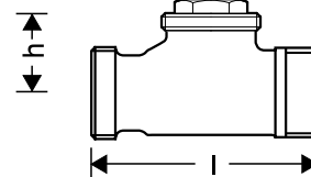
Fig. 8. Straight with external threads
